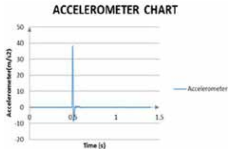
Figure 5. Chart of accelerometer CH0
