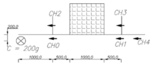
Figure 16. Test layout
