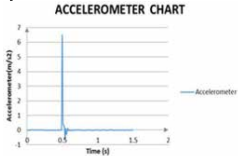
Figure 13. Chart of acceleration meter CH1
